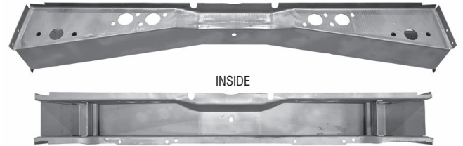
40-10-38-11 MK1 Front Subframe Support (Front Cross Member)
